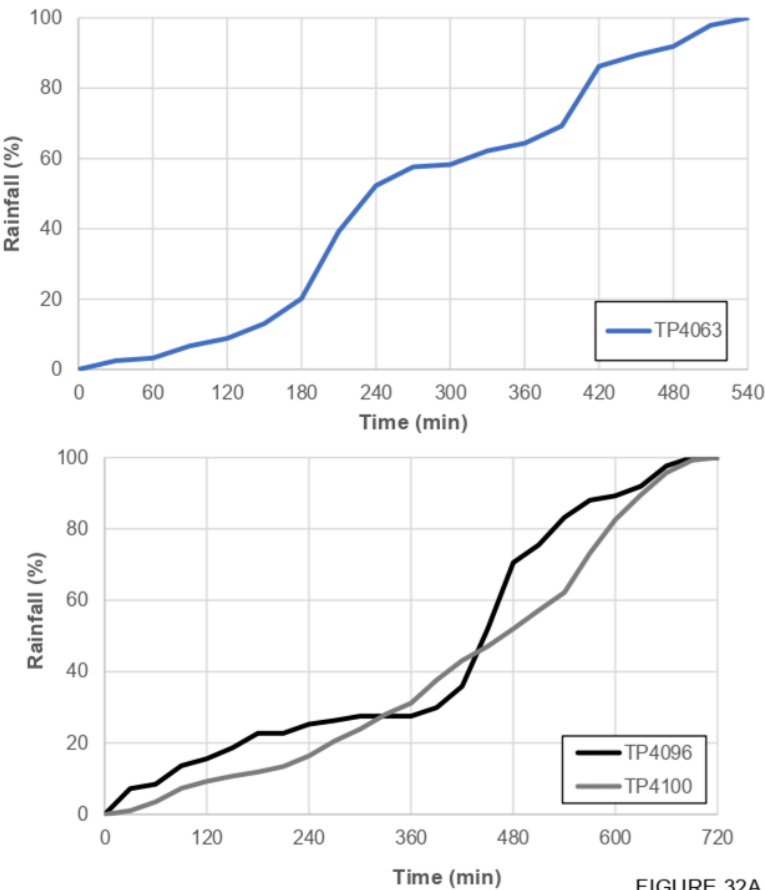
FIGURE 32A ADOPTED DURATIONS AND TEMPORAL PATTERNS FOR DESIGN FLOOD EVENTS MAINSTREAM FLOODING
