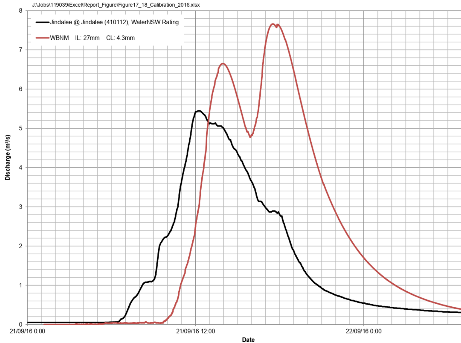
FIGURE 18 HYDROGRAPH AT JINDALEE CREEK AT JINDALEE STATION SEPTEMBER 2016 - WBNM MODEL VS RECORDED HYDROGRAPH
