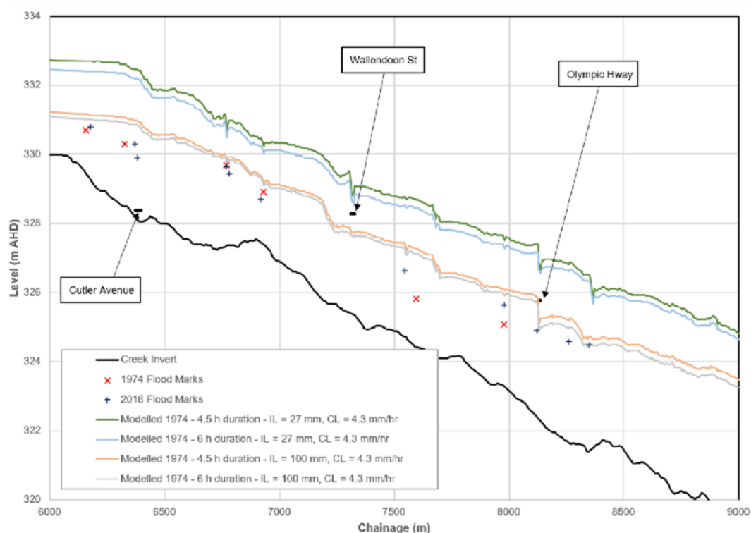
Diagram 3 Muttama Creek Long Section 1974 Event
