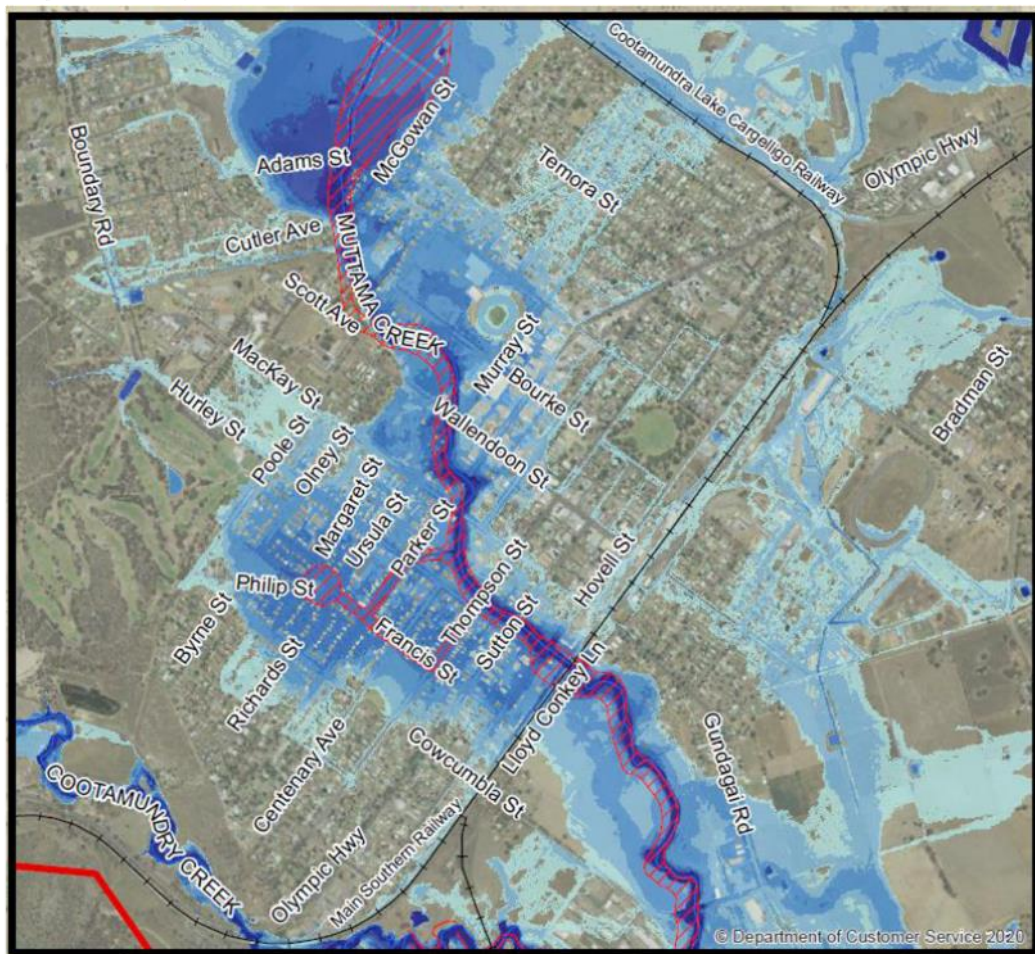
Diagram 4: Comparison of 1% AEP Flood Extent
