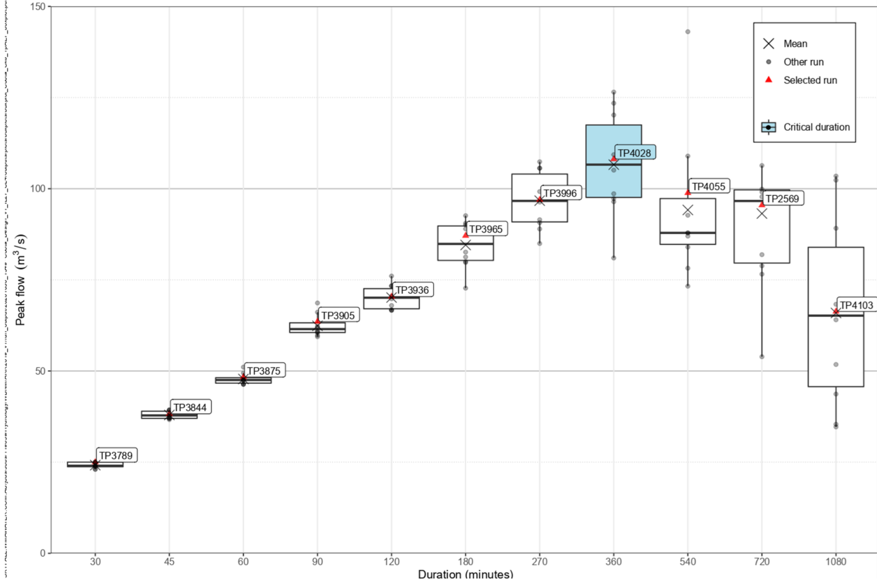
FIGURE 31 Subcatchment: Coota_Ckl 1% AEP Even
