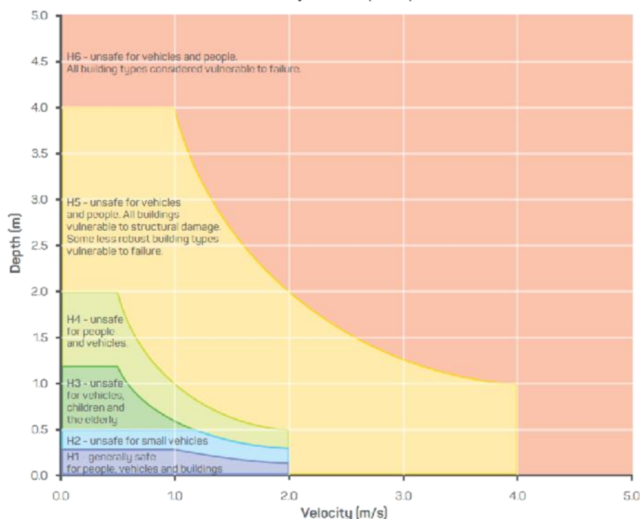
Diagram 6: General flood hazard vulnerability curves (ADR)
