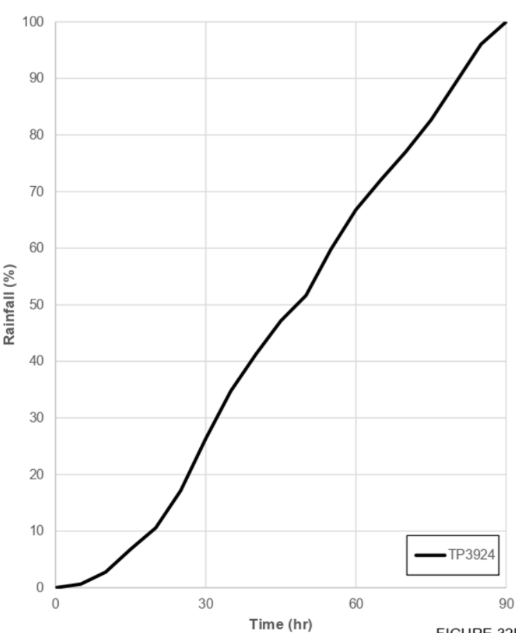
FIGURE 32B ADOPTED DURATIONS AND TEMPORAL PATTERNS FOR DESIGN FLOOD EVENTS OVERLAND FLOODING
