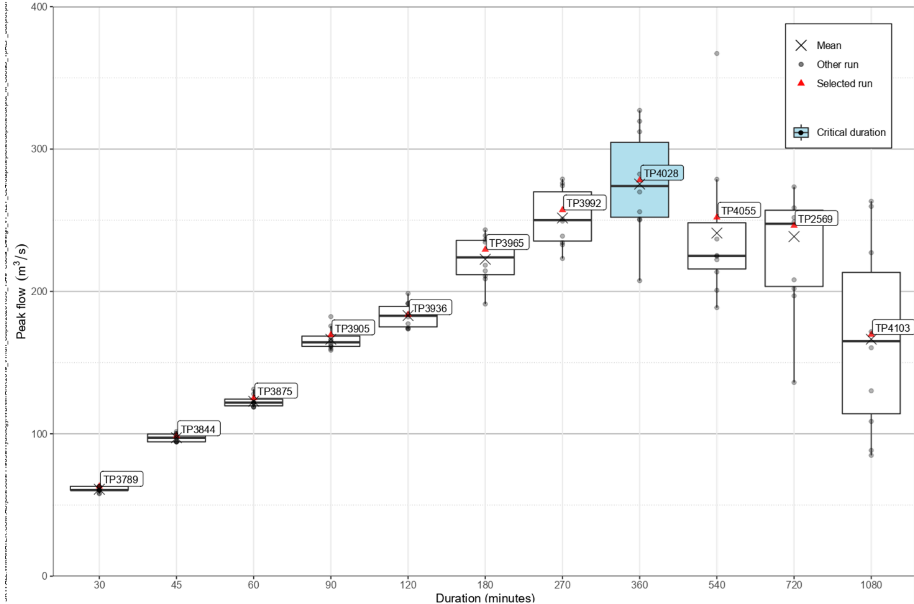
FIGURE 30 Subcatchment: M_Coota: 1% AEP Even
