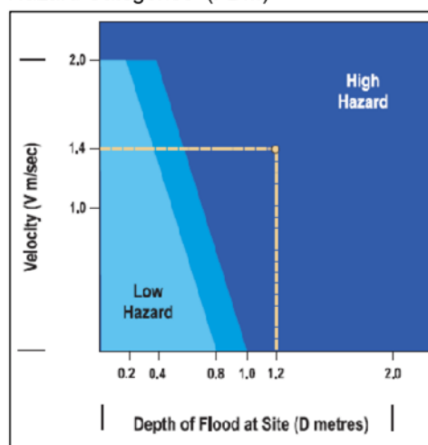
Diagram 5: "L2" Hydraulic Hazard Categories (FDM)
